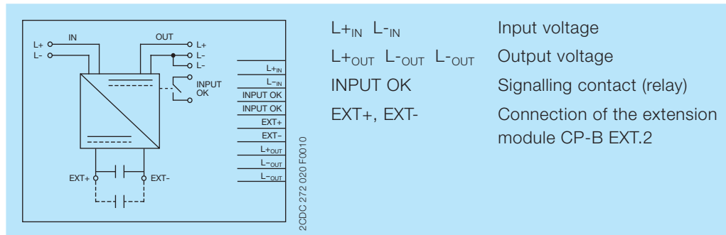
Connection diagram
